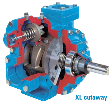
XL cutaway
